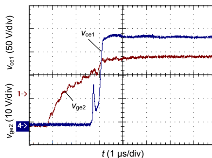
Fig. 14 Pseudo turn-on problem with the BPTM method
