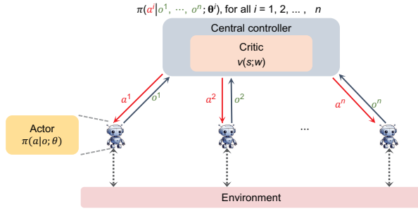
Fig. 2 During training, agents collaboratively learn with access to global state information using a centralized method. During execution, agents independently make decisions using only their local information
