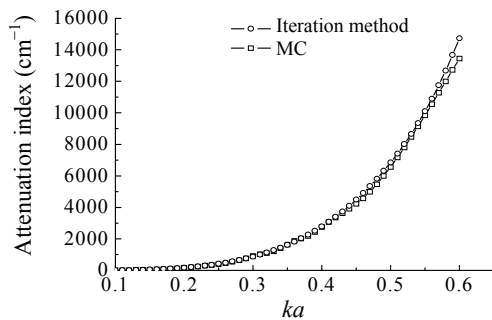
Fig.2 Comparison of MC and iteration method. Fraction volume \eta is 0.25. Number of spheres is 950. Radius of spheres a is 20 nm. Permittivity of spheres \epsilon_\gamma is 13.0 and the refractive index of the matrix is 1.42. Number of iterations is 6
