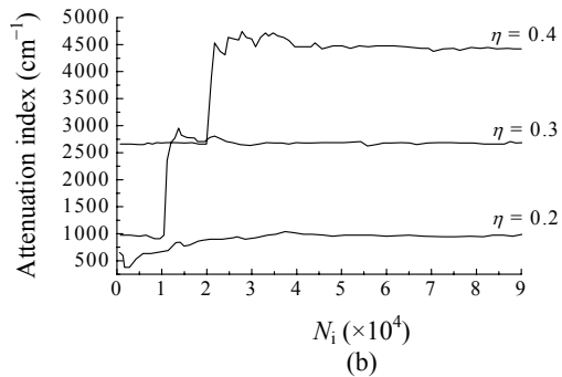
Fig.1 Convergence of attenuation index \tau versus N_i , number of incident photons with fraction volume \eta=0.2, 0.3, 0.4 while the number of spheres is 750, 1100, 1500, respectively. The radius of spheres is 20 nm. The permittivity of the spheres is 13.0 and the refractive index of the matrix is 1.42. The ka of (a) and (b) is 0.2 and 0.4, respectively
