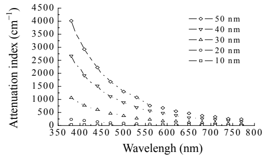
Fig.3 Spectra of attenuation index according to silicon crystallites in c-Si/ \alpha -Si matrix. Permittivity of spheres is 13.0 and the refractive index of the matrix is 1.42. Diameter of spheres ranges from 10 nm to 50 nm. Fraction volume \eta is 0.5
