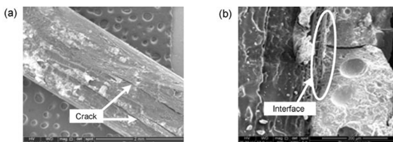
Fig. 10 Interface condition after treatment at a high temperature of 200 °C for 90 min
