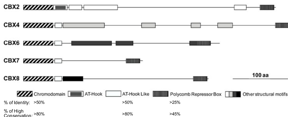
Fig. 2 Domain organization and conservation among CBX proteins
