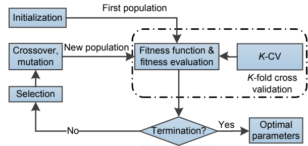
Fig. 3 The flowchart of KSVM parameter optimization using GA
