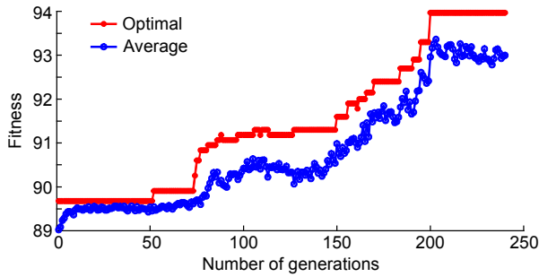
Fig. 5 The curve of fitness vs. different numbers of generations using the GA method ( K=4 , terminal generation=240, population size=30)
