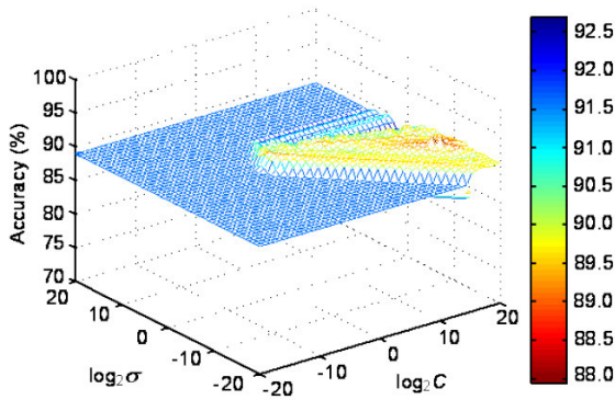
Fig. 6 The 3D view of optimization parameters using the GS method
