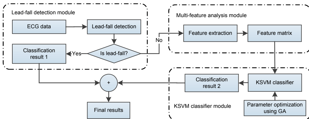
Fig. 1 The flowchart of the proposed method which includes three modules
