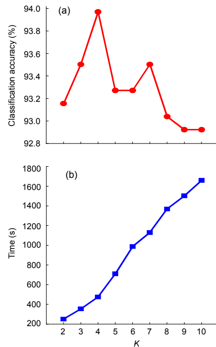
Fig. 4 The corresponding classification accuracy for set C using K -CV (a) and the time cost (b) with the increase of K
