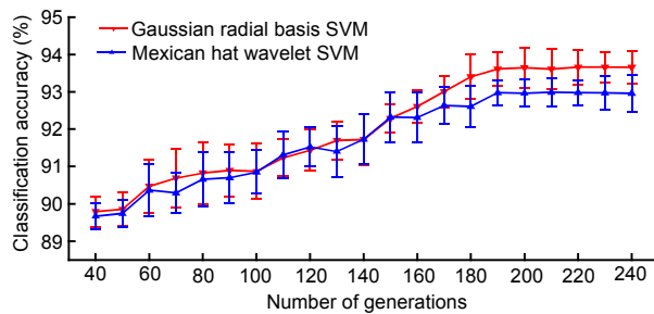
Fig. 7 Comparison of classification accuracy between the Gaussian radial basis SVM and Mexican hat wavelet SVM
